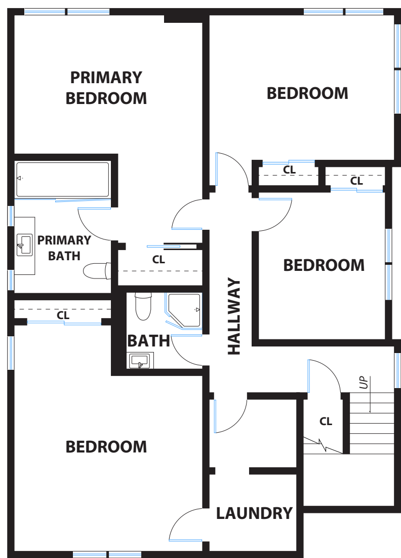
MAIN LEVEL
